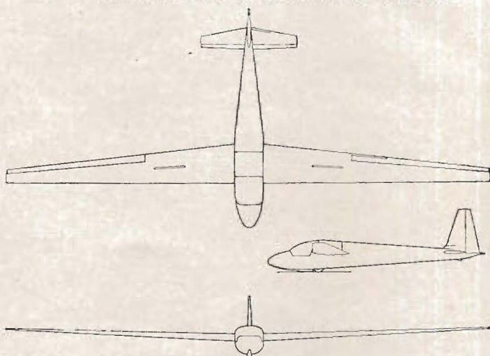
Fig. 12.—Crabpot I—Design 30: general arrangement
