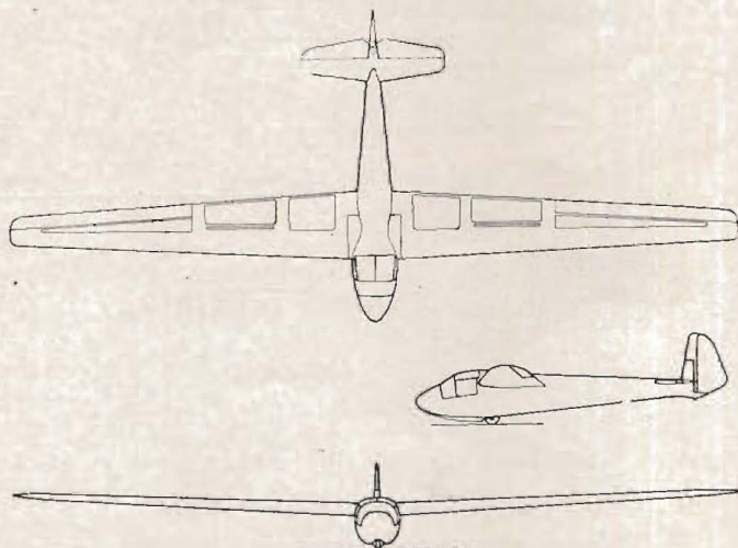
Fig. 13.—Design 39: general arrangement
