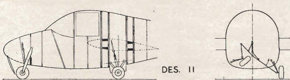
Fig. 11.—Retractable undercarriages. Hi 21 and Design II
